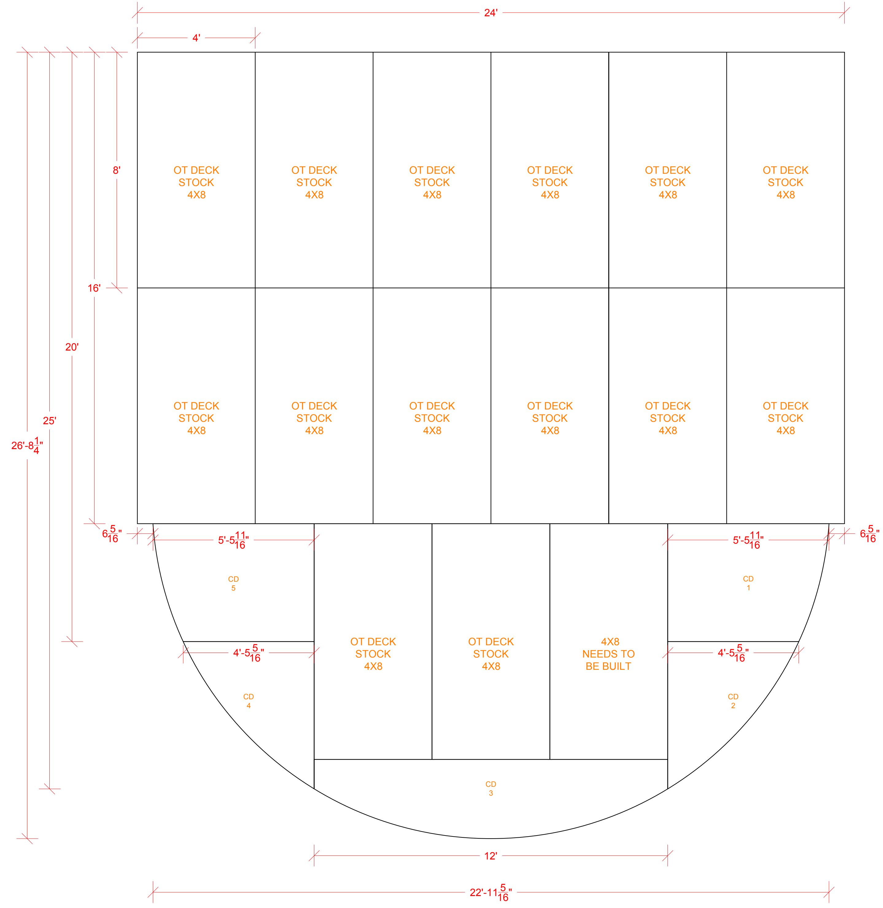
DECK 3
